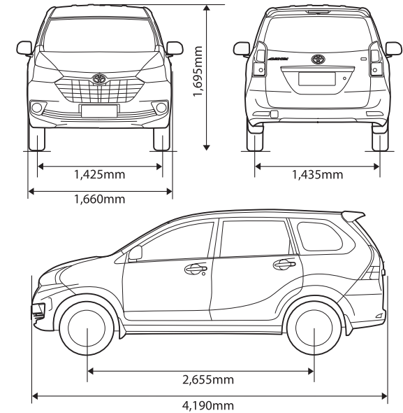
Dimensions shown are based on 1.5G variant.
